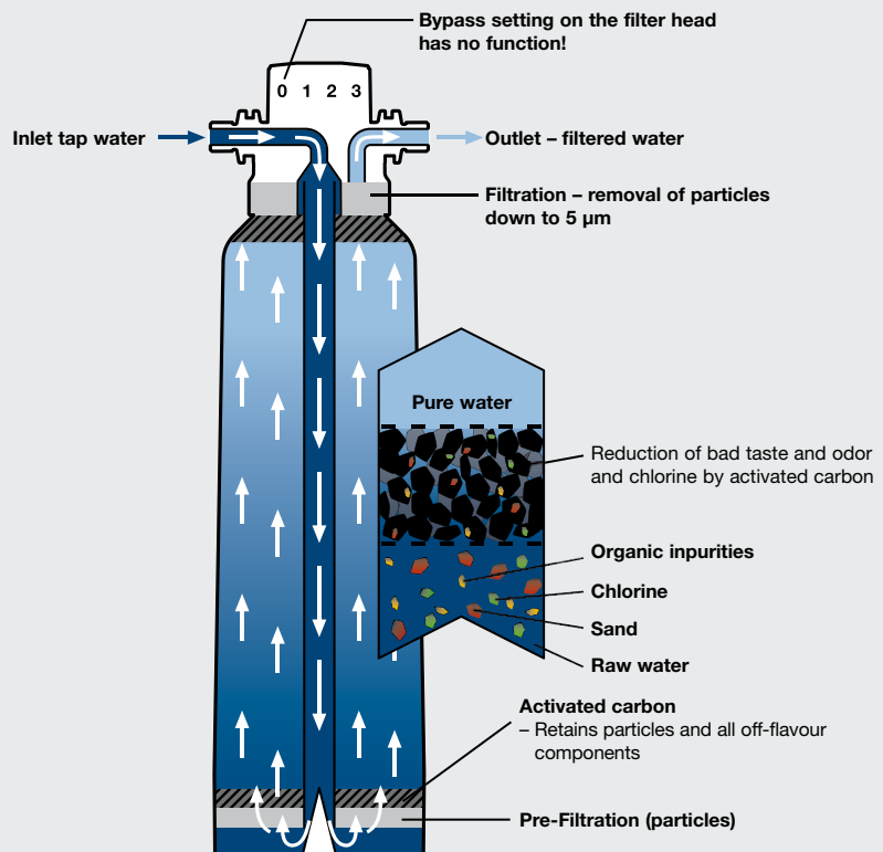
Cross-Section of a besttaste filter cartridge
